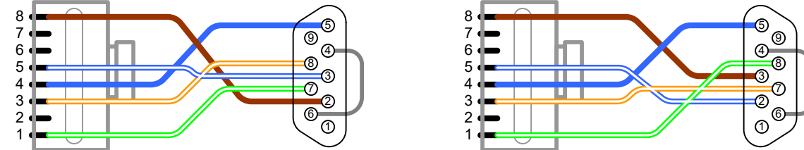
Wire entry view (i.e., opposite of mating side) shown for all connectors; TIA T568A wire colors shown
