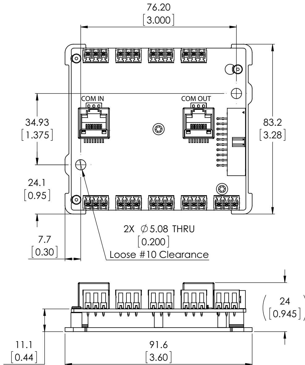
CCIO-8 Mounting Dimensions
