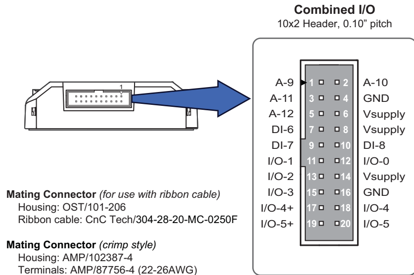
ClearLink I/O Header
