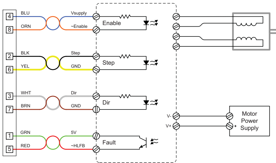
Stepper motor drive wired to ClearLink controller
